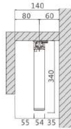
Single straight track installation
