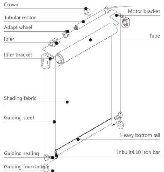
Motorized Roller Blind (Guiding steel) structural drawing
