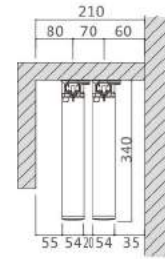
Double straight track installation
