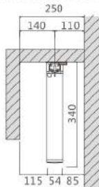
Single curved track installation
