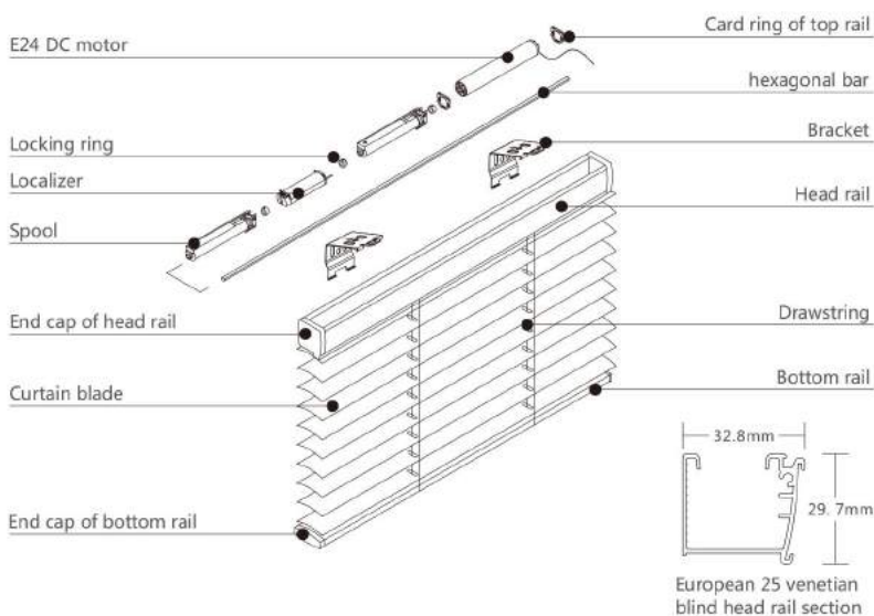
E24 Venetian Blind organization chart
