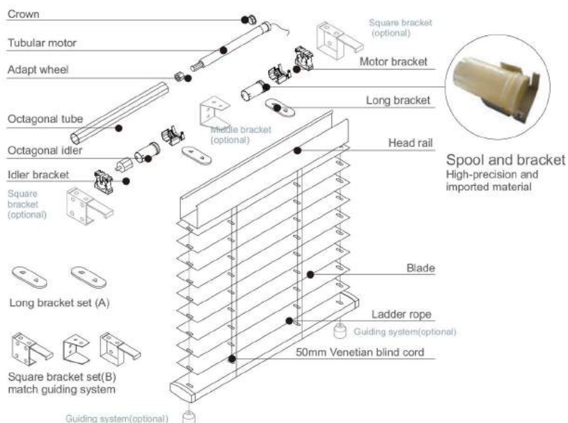
50mm Wooden Venetian Blind structural drawing
