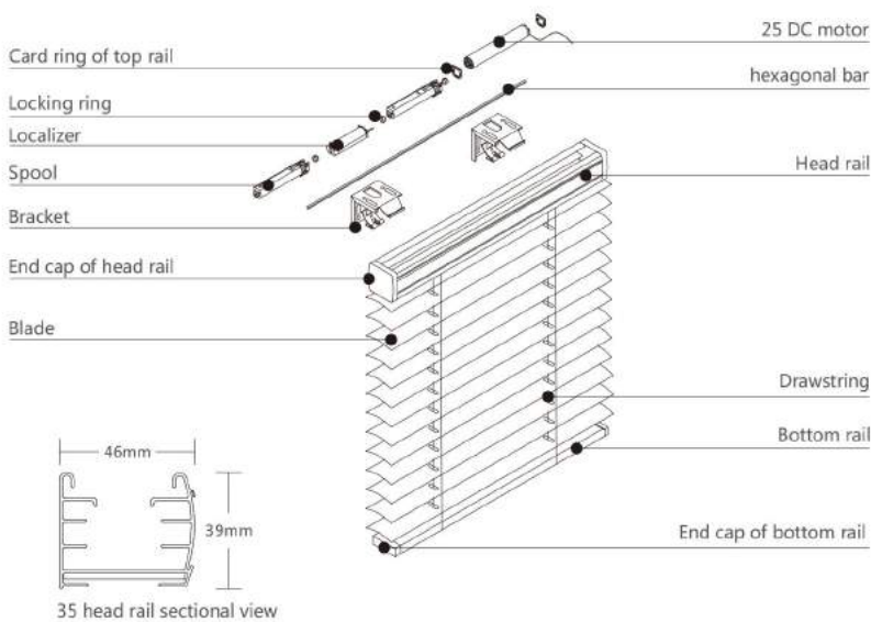
35mm Venetian Blind structure chart
