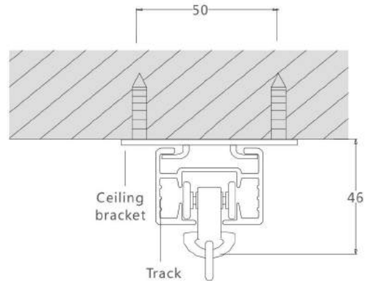
Top installation
