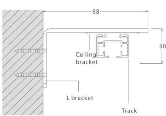
Side installation
