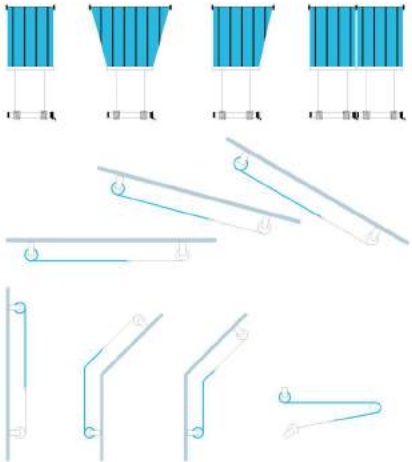
FSS skylight (installation method)
