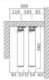
Double curved track installation
