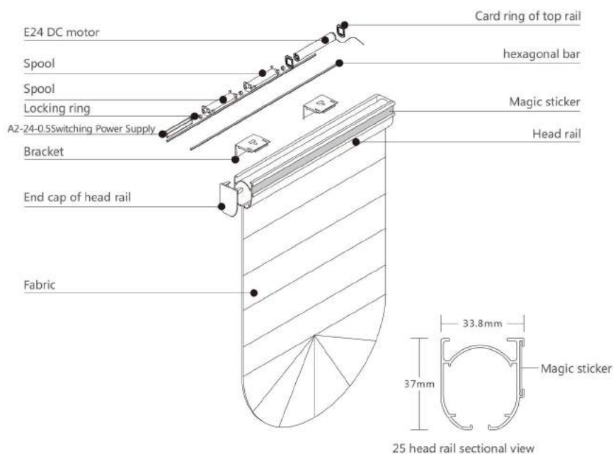
Light Roman Blind structure chart
