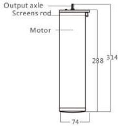
Motor size
