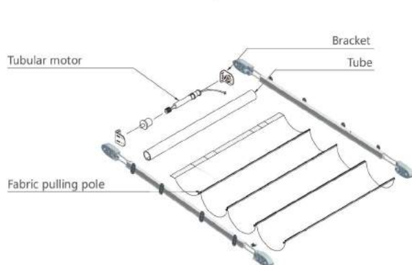
Skylight Shade
