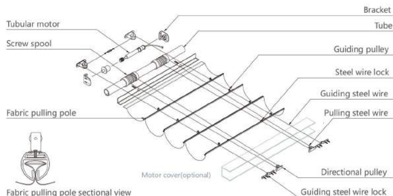
FCS Folding Skylight Shade (Steel wire guiding)
